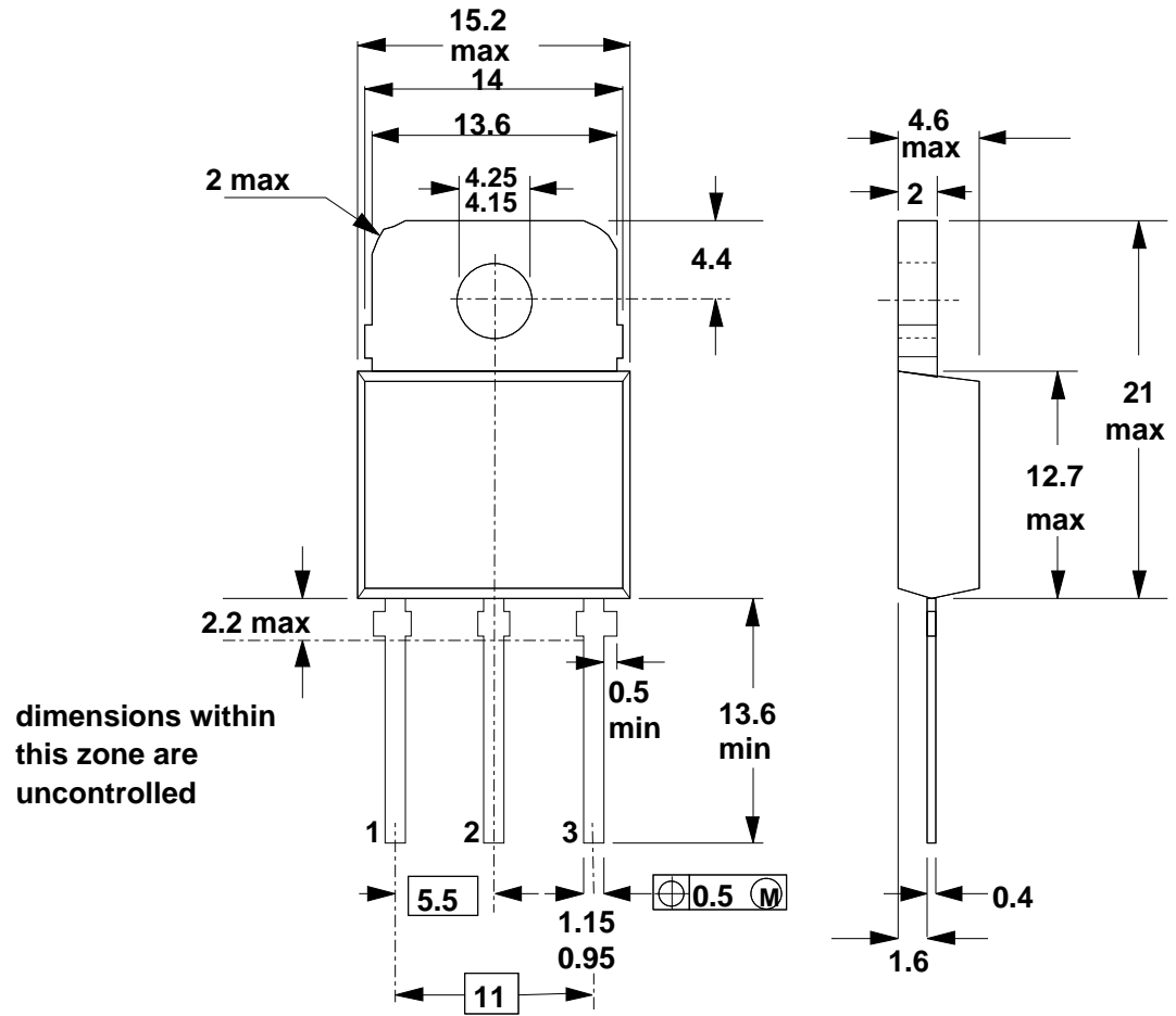
Fig.7. SOT93; pin 2 connected to mounting base.
