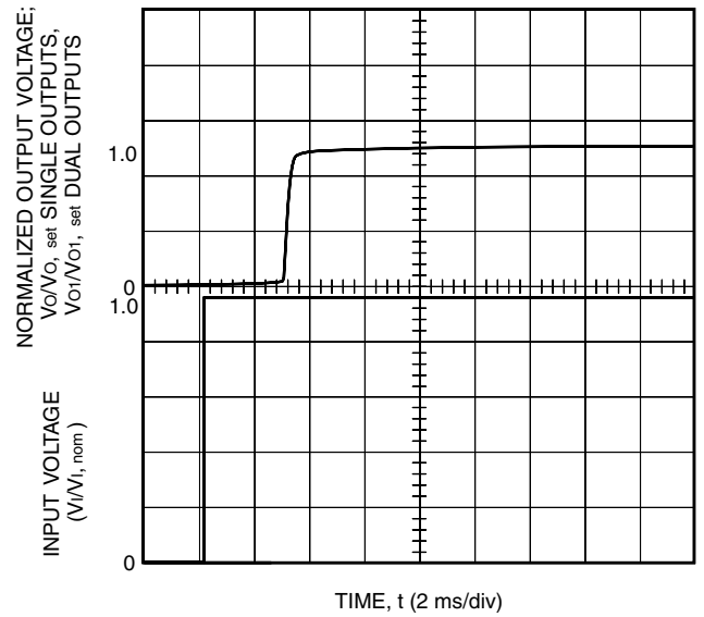
Figure 31. Typical Output Voltage Start-Up when Input Voltage Is Applied; I_o = 80\% of I_{o, max} , V_i = Nominal Line
