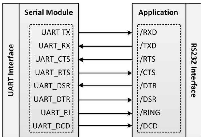
Figure 3: UART Interfaces
