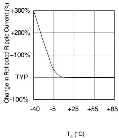
REFLECTED RIPPLE CURRENT vs TEMPERATURE
