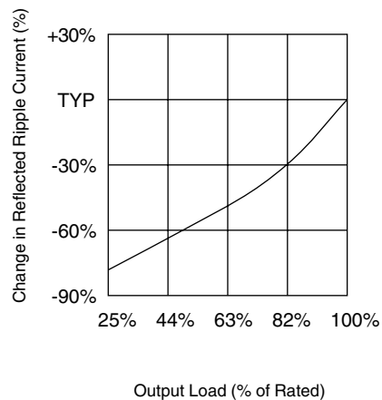
REFLECTED RIPPLE CURRENT vs OUTPUT LOAD
