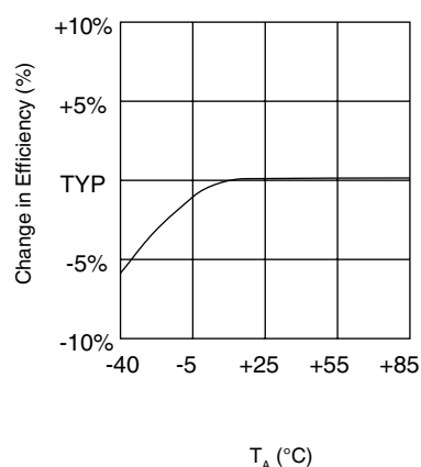
EFFICIENCY vs TEMPERATURE
