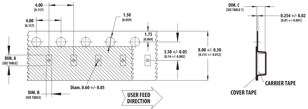
Figure 8. Tape Dimensions
