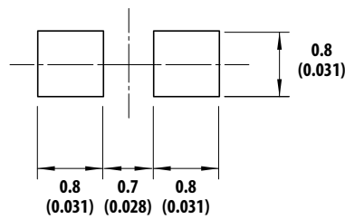
Figure 6. Recommended soldering land pattern
