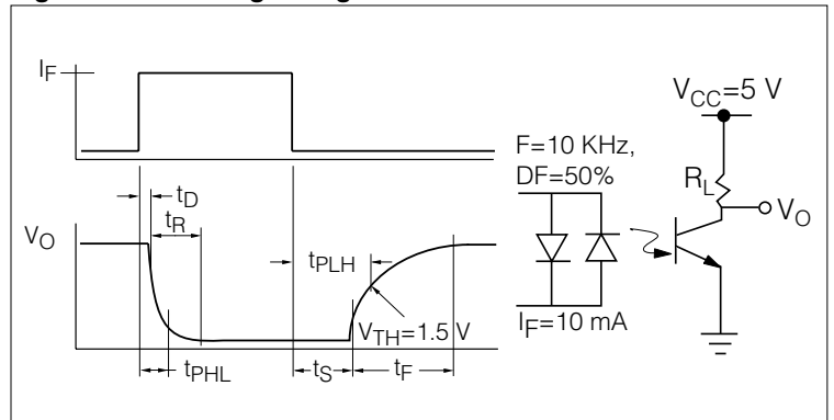
Figure 14. Switching timing and schematic
