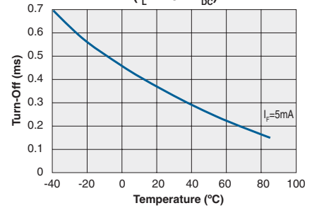
Typical Turn-Off vs. Temperature ( I_L=170mA_{DC} )
