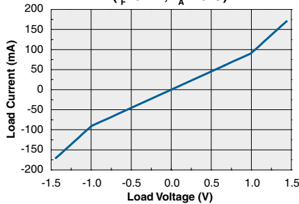
Typical Load Voltage vs. Load Current ( I_F=5mA , T_A=25°C )
