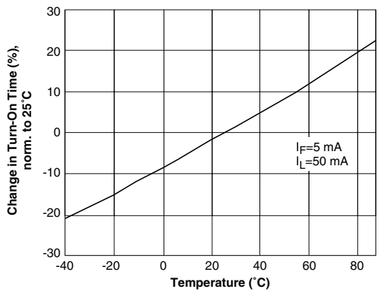
Figure 18. Turn-On Time vs. Temperature
