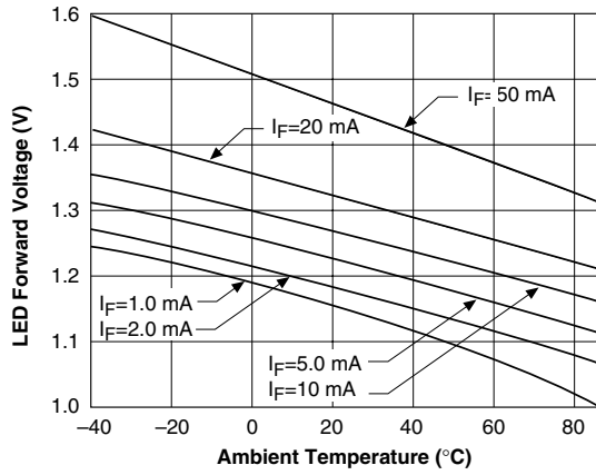
Figure 1. LED Voltage vs. Temperature
