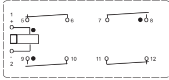
Bottom view The contacts are shown in the deenergized condition.
