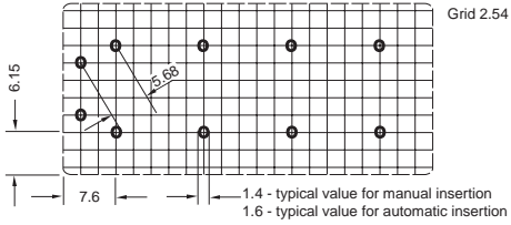
Bottom view The contacts are shown in the deenergized condition.
