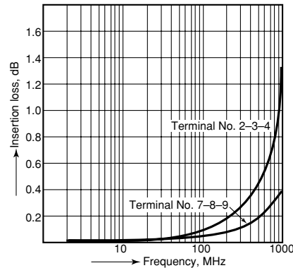
15-(2). High-frequency characteristics
