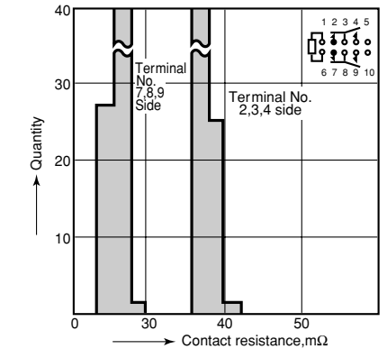
11. Distribution of contact resistance
