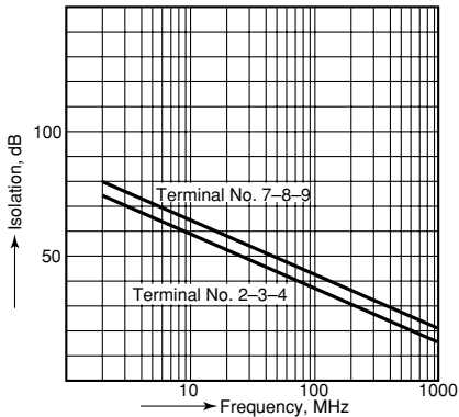
15-(1). High-frequency characteristics
