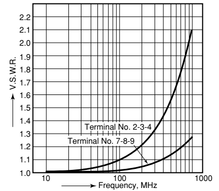
15-(3). High-frequency characteristics
