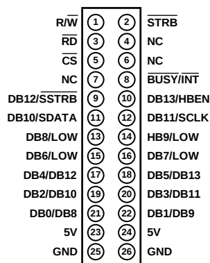
Figure 27. SKT4 Pinout
