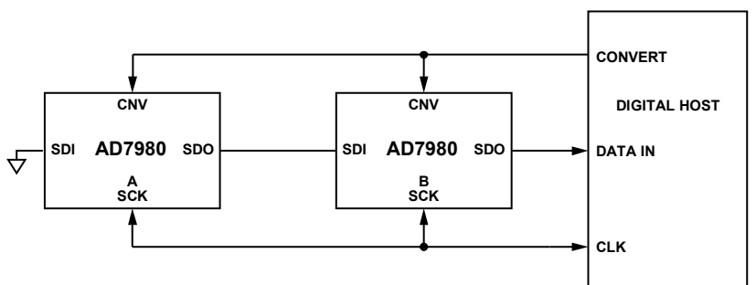
Figure 39. Chain Mode Without Busy Indicator Connection Diagram
