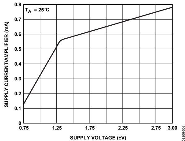
Figure 8. Supply Current per Amplifier vs. Supply Voltage
