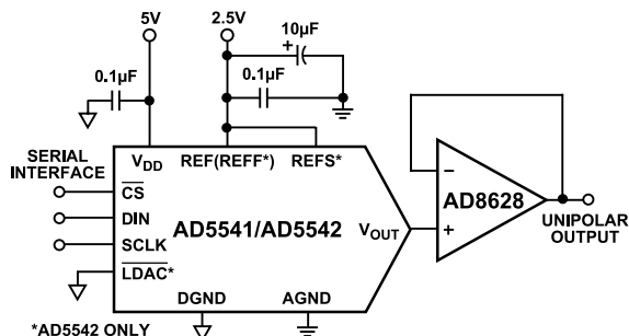
Figure 64. AD8628 Used as an Output Amplifier
