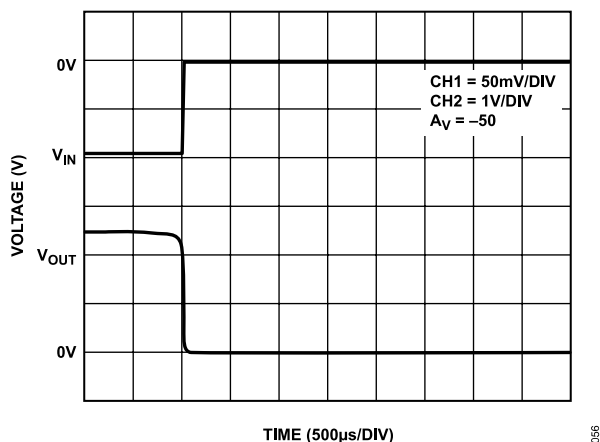
Figure 59. Negative Input Overload Recovery for the AD8628
