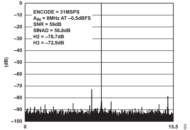
Figure 23. FFT: FS = 31 MSPS, A_{IN} = 8\text{ MHz @ } -0.5\text{ dBFS} , Differential, with AD8138 Driving ADC Inputs, 1 V p-p Input Range
