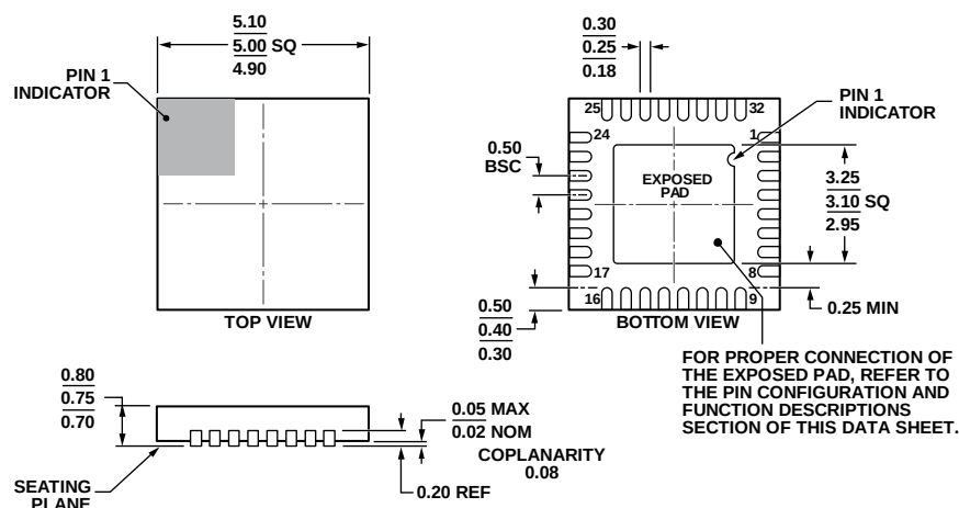
Figure 37. 32-Lead Lead Frame Chip Scale Package [LFCSP_WQ] 5 mm x 5 mm Body, Very Very Thin Quad (CP-32-7)
