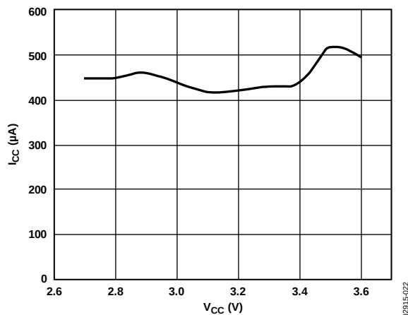
Figure 22. I_{CC} vs. V_{CC} (Unloaded)
