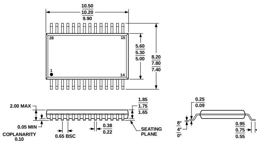
Figure 38. 28-Lead Shrink Small Outline Package [SSOP] (RS-28)
