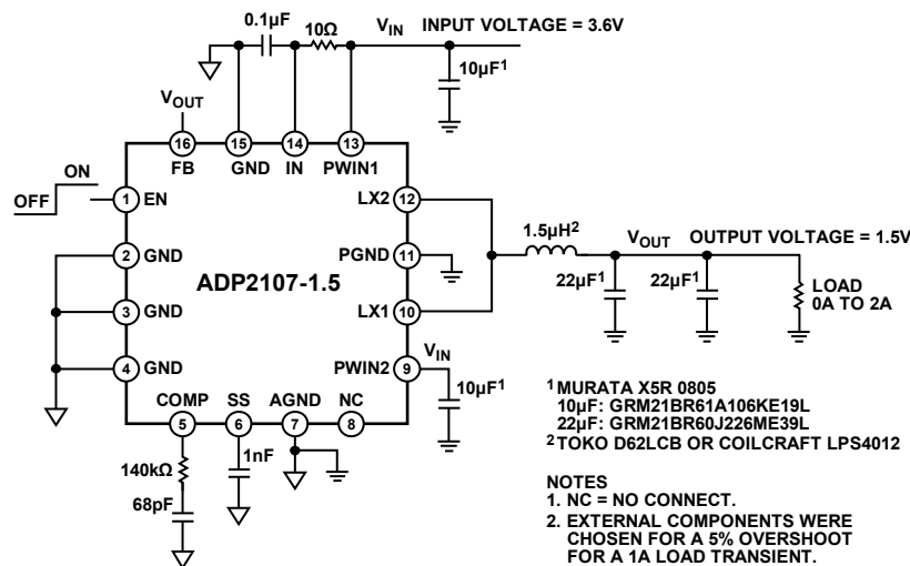
Figure 57. Application Circuit— V_{IN} = 3.6\text{ V} , V_{OUT} = 1.5\text{ V} , Load = 0 A to 2 A
