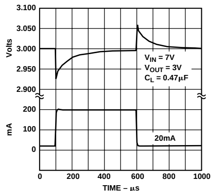
Figure 13. Load Transient Response
