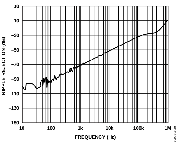
Figure 28. Ripple Rejection
