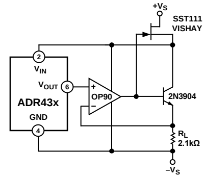
Figure 36. High Voltage Floating Current Source
