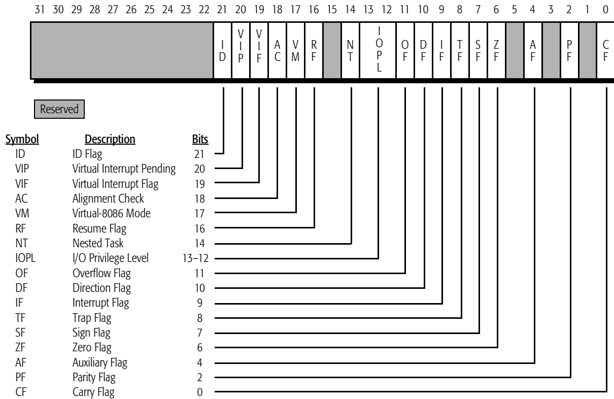
Figure 20. EFLAGS Registers
