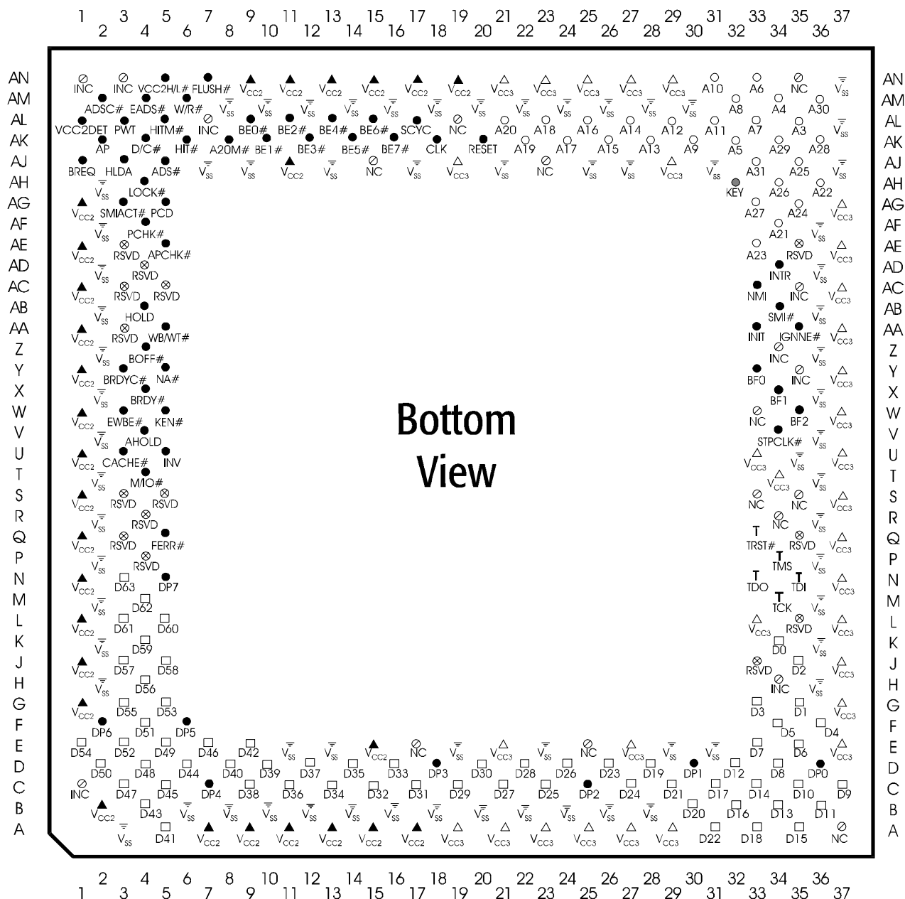
Figure 113. AMD-K6 ® -2 Processor Pin-Side View
