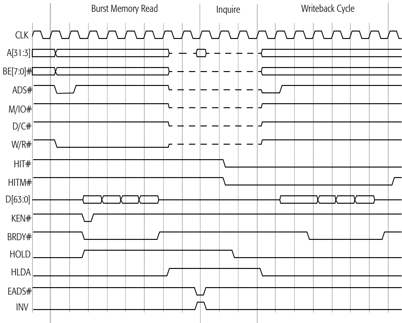
Figure 63. HOLD-Initiated Inquire Hit to Modified Line
