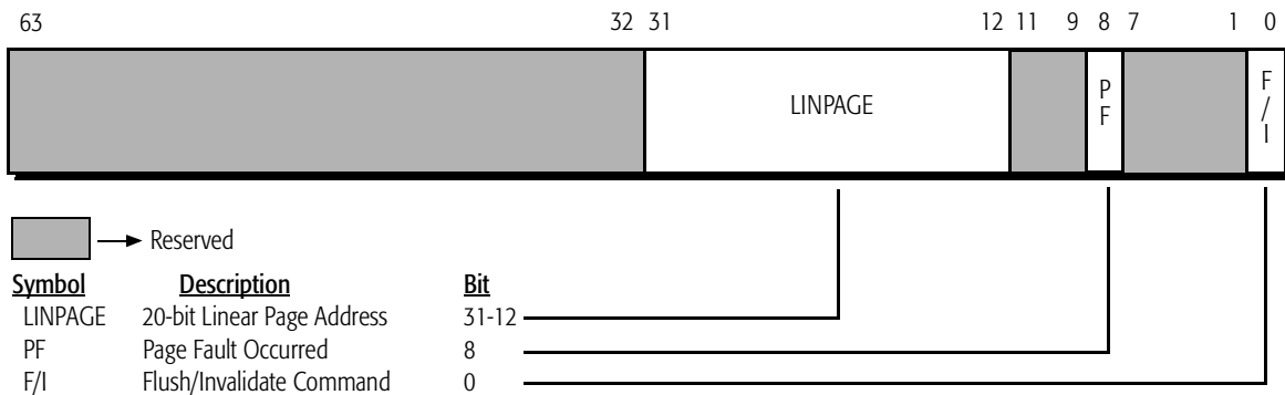
Figure 51. Page Flush/Invalidate Register (PFIR)
