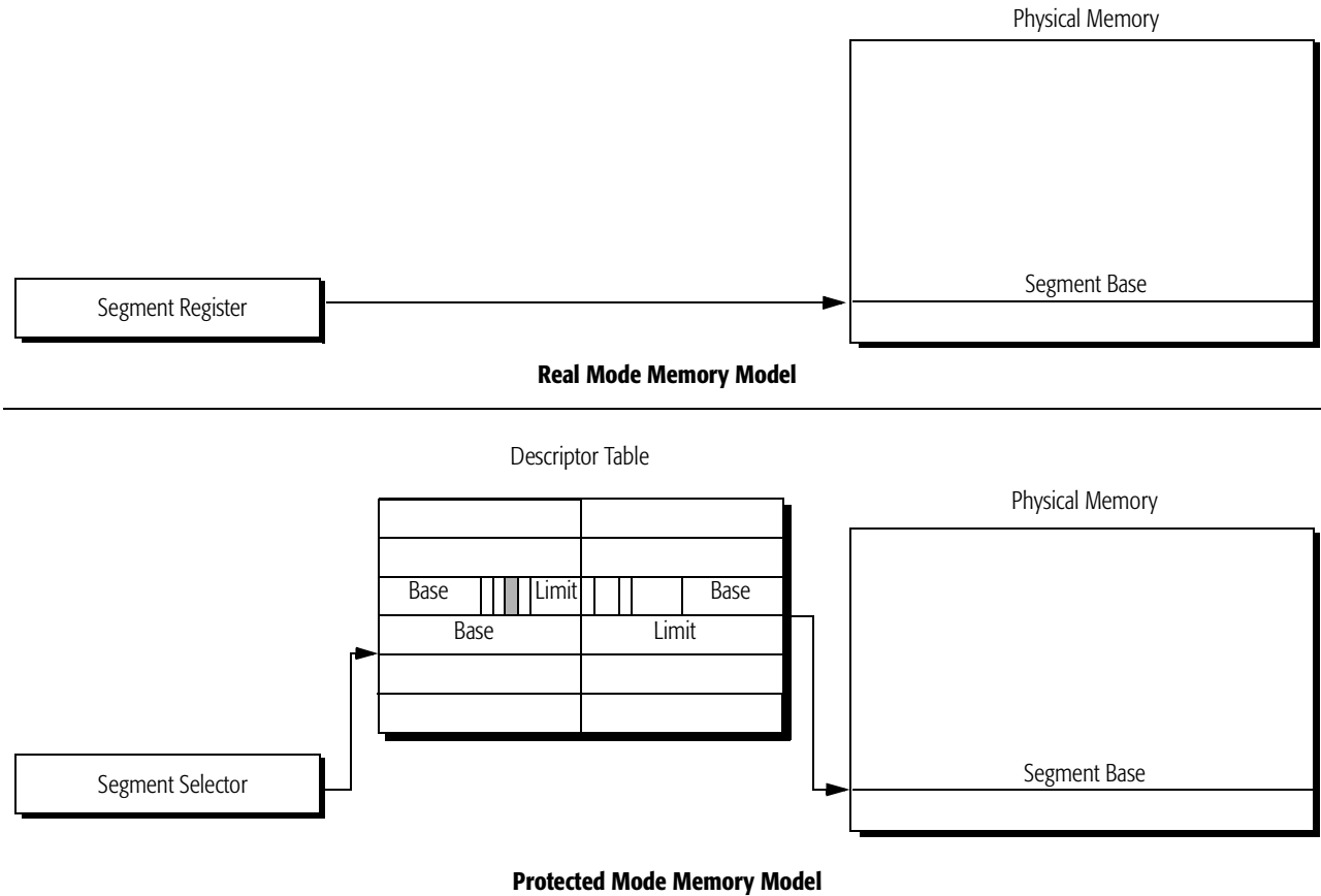
Figure 10. Segment Usage
