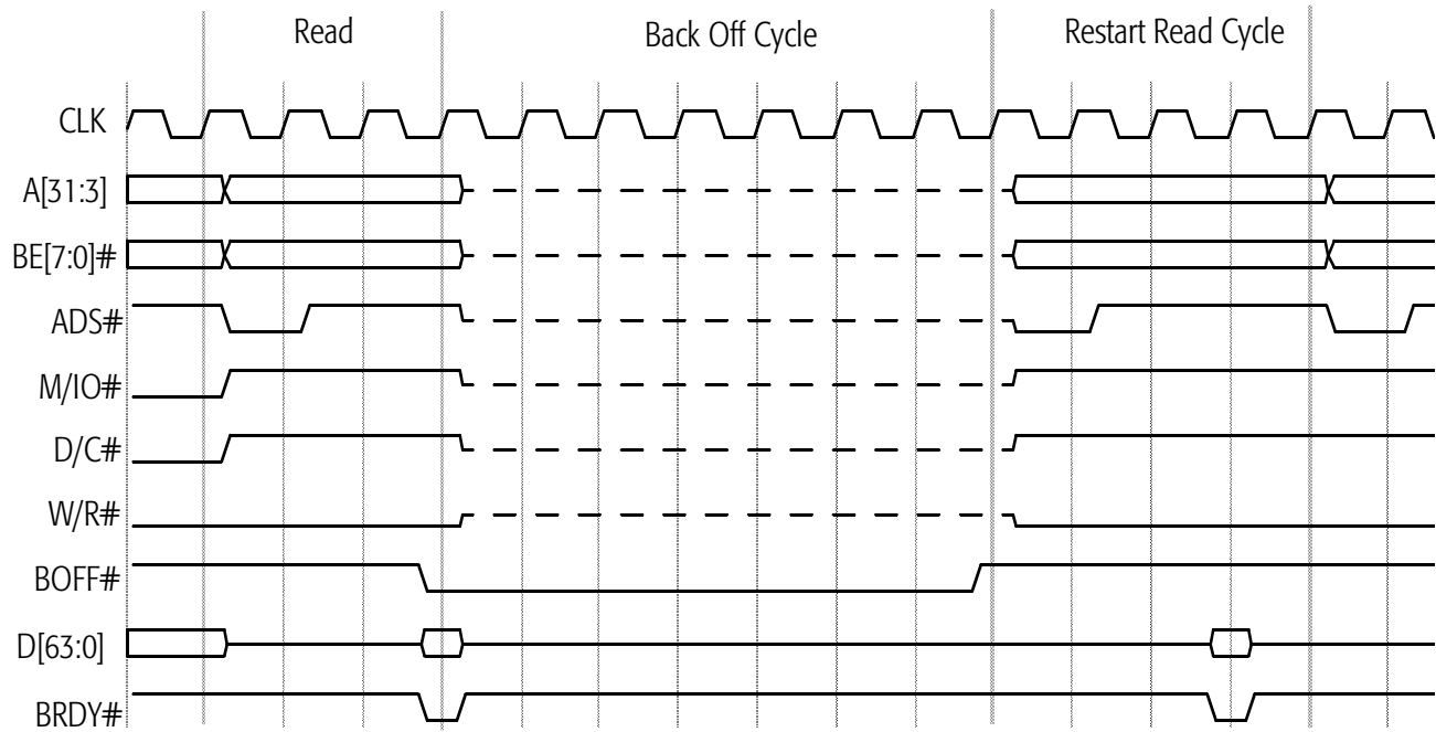
Figure 68. BOFF# Timing
