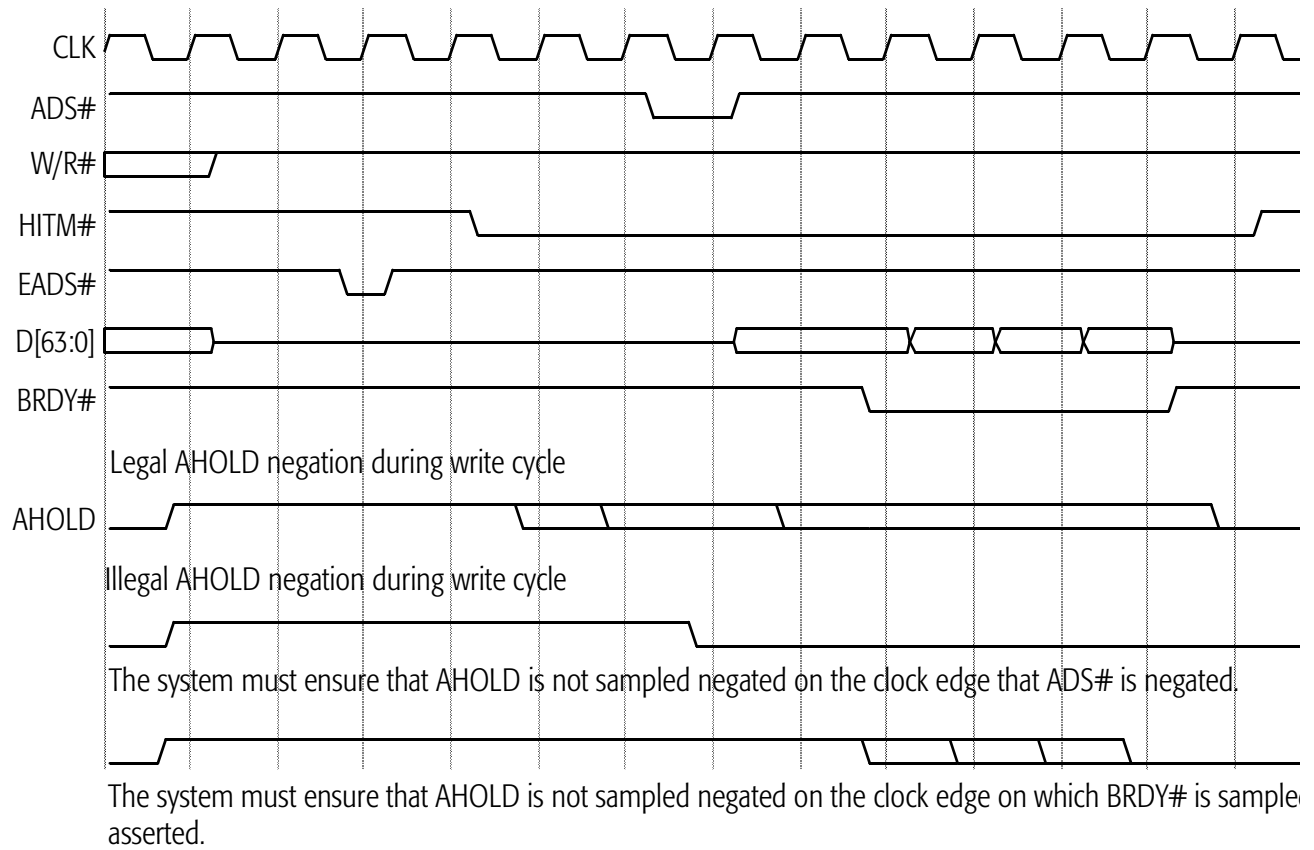
Figure 67. AHOLD Restriction
