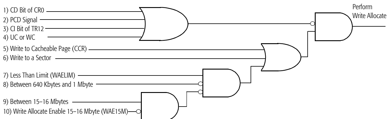
Figure 81. Write Allocate Logic Mechanisms and Conditions
