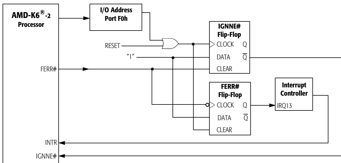
Figure 84. External Logic for Supporting Floating-Point Exceptions
