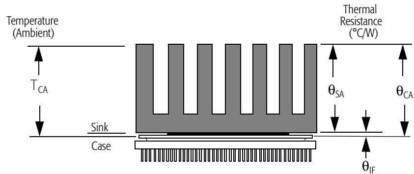
Figure 104. Thermal Model
