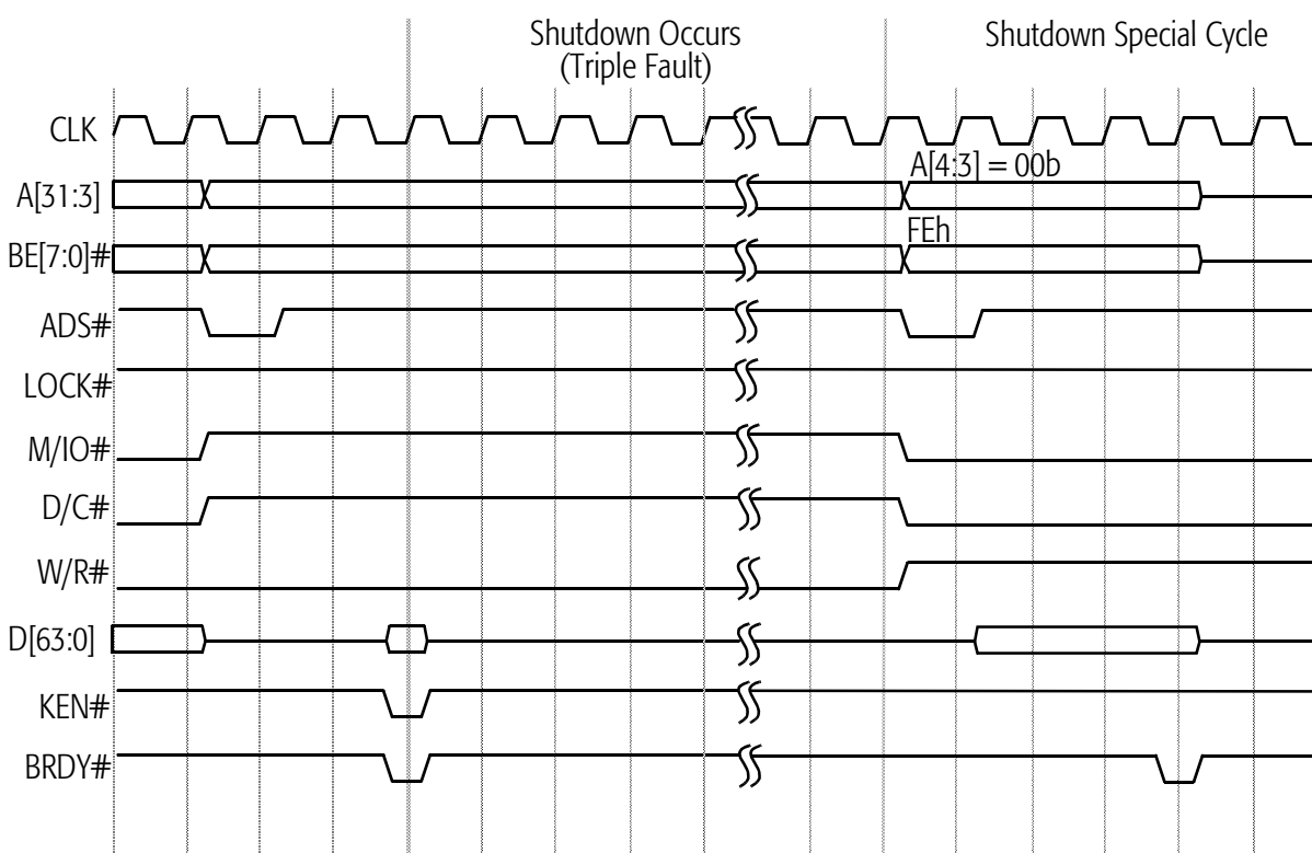
Figure 73. Shutdown Cycle
