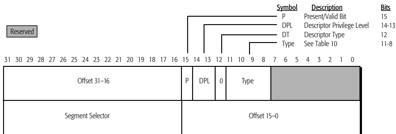
Figure 46. Gate Descriptor
