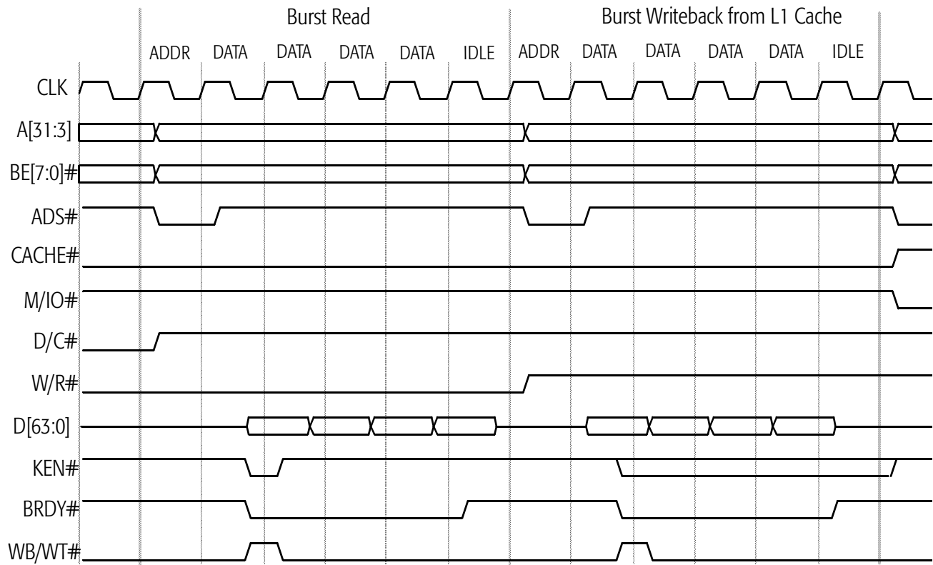
Figure 58. Burst Writeback due to Cache-Line Replacement
