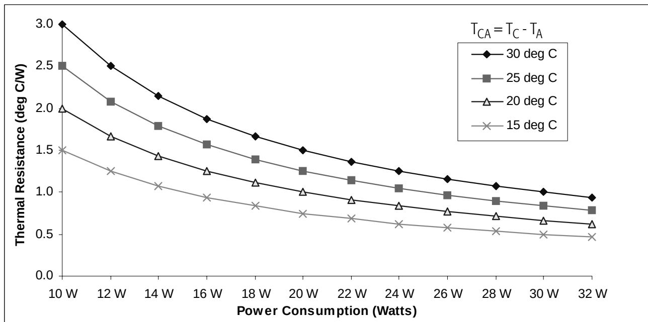
Figure 105. Power Consumption versus Thermal Resistance
