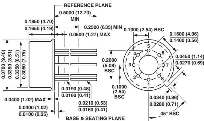
8-Lead Metal Can [TO-99] [J Suffix] (H-08B)
