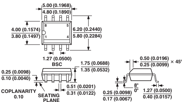
8-Lead Small Outline Package [SOIC] [S Suffix] (R-8)
