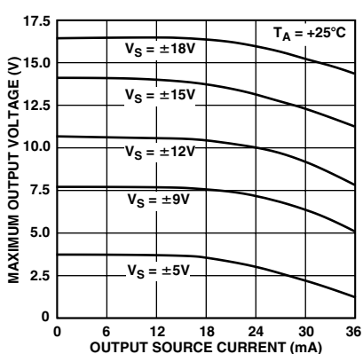
TPC 14. Maximum Output Voltage vs. Output Current (Source)
