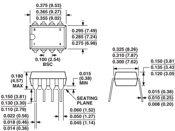
8-Lead Plastic Dual In-Line Package [PDIP] [P Suffix] (N-8)
