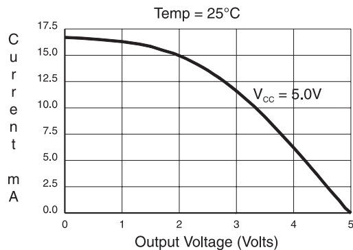
OUTPUT SOURCE CURRENT vs. OUTPUT VOLTAGE
