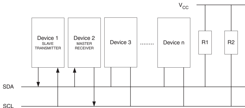
Figure 15-17. Data Transfer in Slave Transmitter Mode
