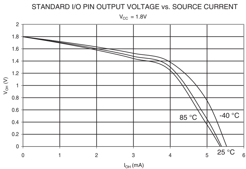
Figure 23-31. V_{OH} : Standard I/O Pin Output Voltage vs. Source Current ( V_{CC} = 1.8V )
