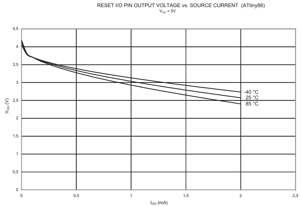
Figure 23-96. V_{OH} : Reset Pin Output Voltage vs. Source Current ( V_{CC} = 5V )
