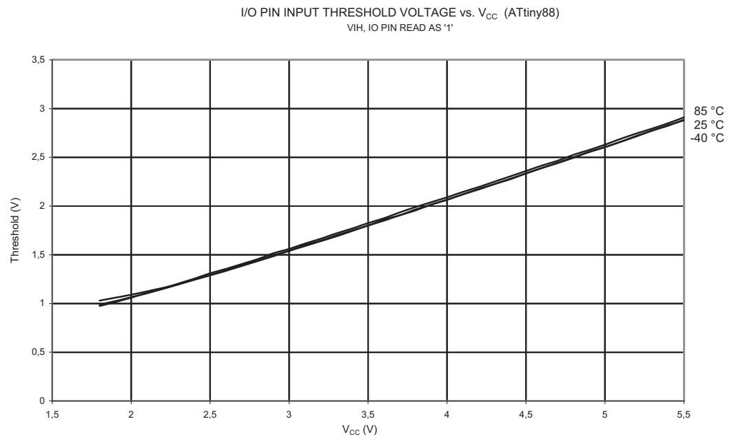
Figure 23-97. V_{IH} : I/O Pin Input Threshold Voltage vs. V_{CC} (IO Pin Read as '1')
