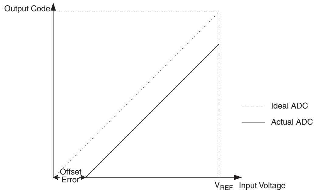
Figure 17-10. Offset Error
