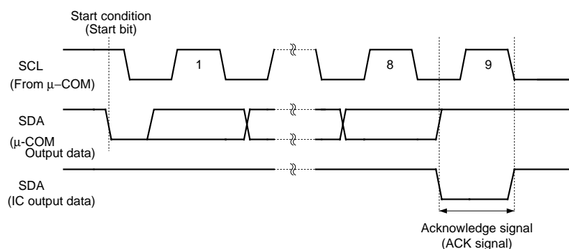
Fig.3 Acknowledge (ACK signal) response (during write and read slave address input)
