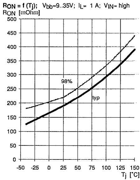
On-state resistance ( V_{bb} -Pin to OUT-Pin)
