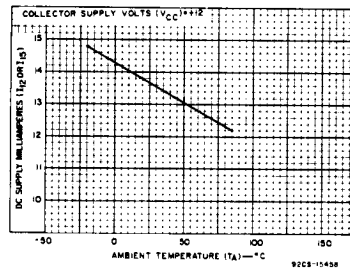
Fig. 5 - Typical DC supply current vs ambient temperature.
