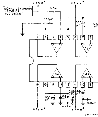
Fig. 13 — Test circuit for measurement of inter-amplifier audio separation "cross talk" characteristic.
