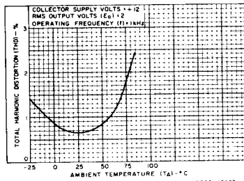
Fig. 10 — Typical total harmonic distortion vs ambient temperature.
