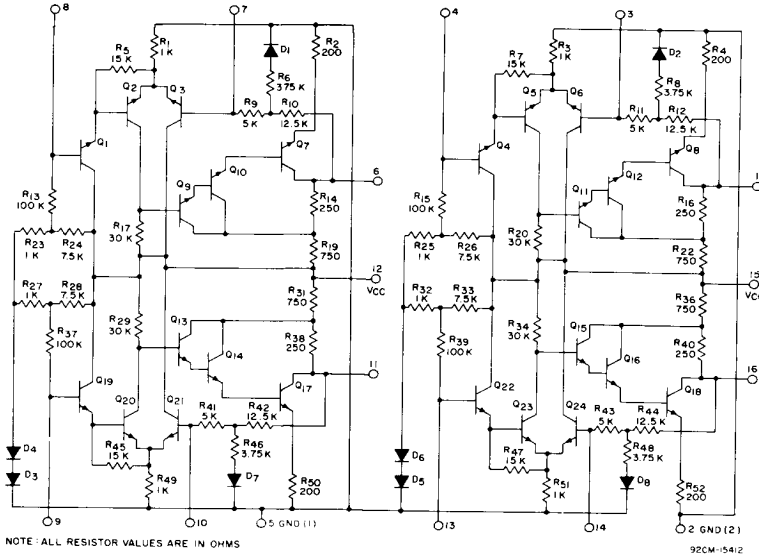
Fig. 3 - Schematic diagram for CA3052.
