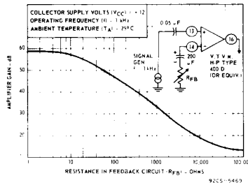
Fig. 15 — Typical amplifier gain vs feedback resistance.
