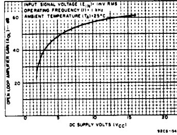
Fig. 7 — Typical amplifier gain vs DC supply voltage.
