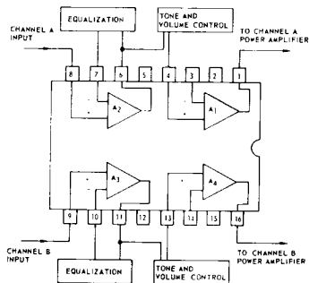
Fig. 1 - Block diagram of stereo preamplifier using CA3052.
