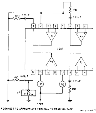
Fig. 4 - Test circuit for measurement of collector supply voltage and currents.
