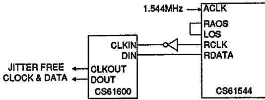
Figure A3. Receiver Jitter Attenuation
