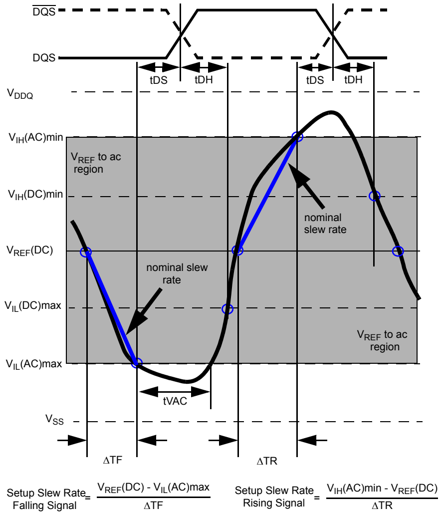
Figure 7. Illustration of nominal slew rate for t_{DS} (differential \overline{DQS}, DQS )
