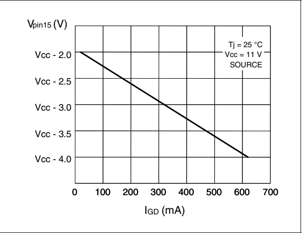
Figure 33. Gate-drive output high saturation
