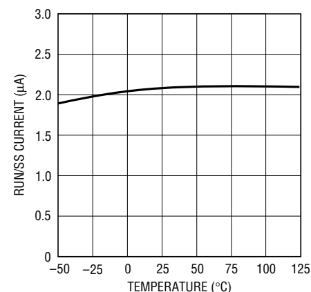
I_{RUN/SS} vs Temperature
