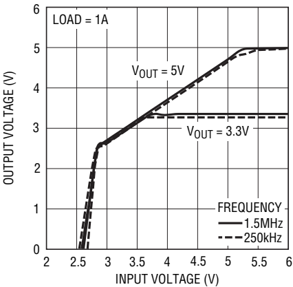
Dropout Operation
