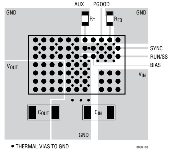
Figure 3. Layout Showing Suggested External Components, GND Plane and Thermal Vias
