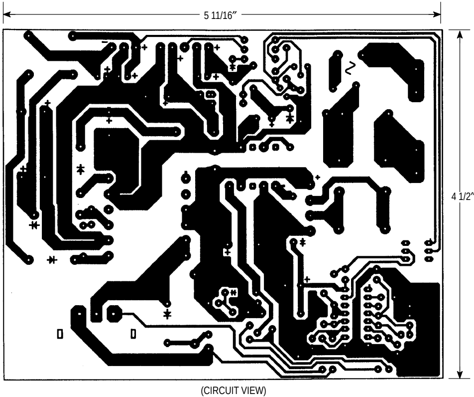
Figure 29. PC Board Circuit Side and Component View
