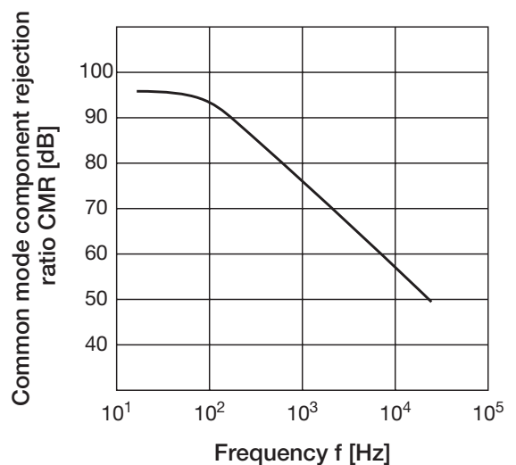
Common mode component rejection ratio vs frequency
