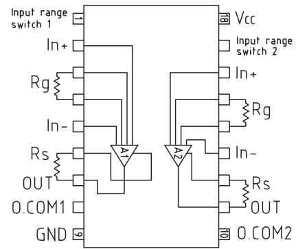
Fig.3. Pinout
