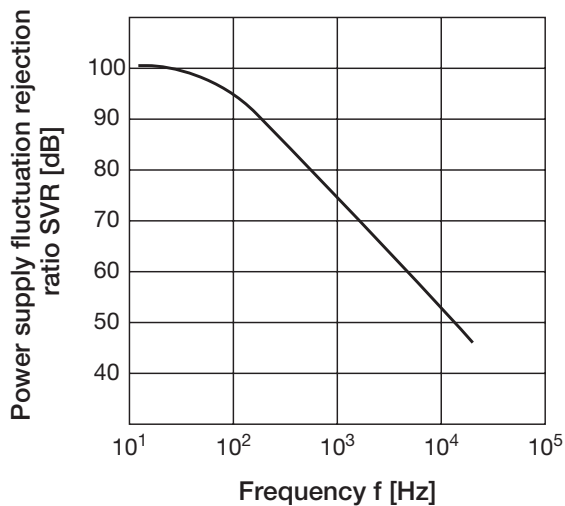
Power supply fluctuation rejection ratio vs frequency
