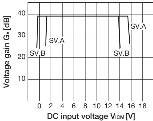
Common-mode input voltage range
