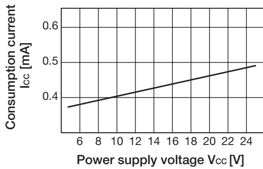
Consumption voltage vs power supply voltage
