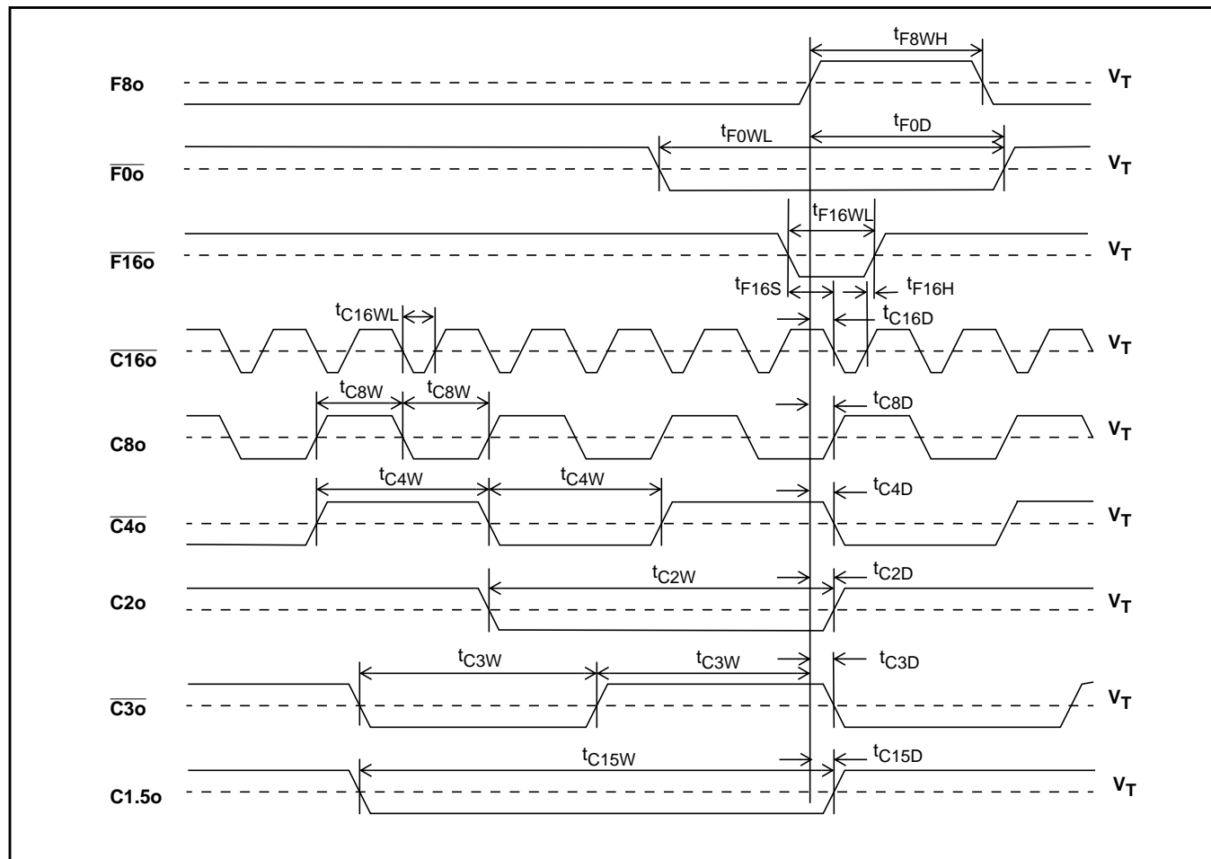
Figure 12 - Output Timing 1
