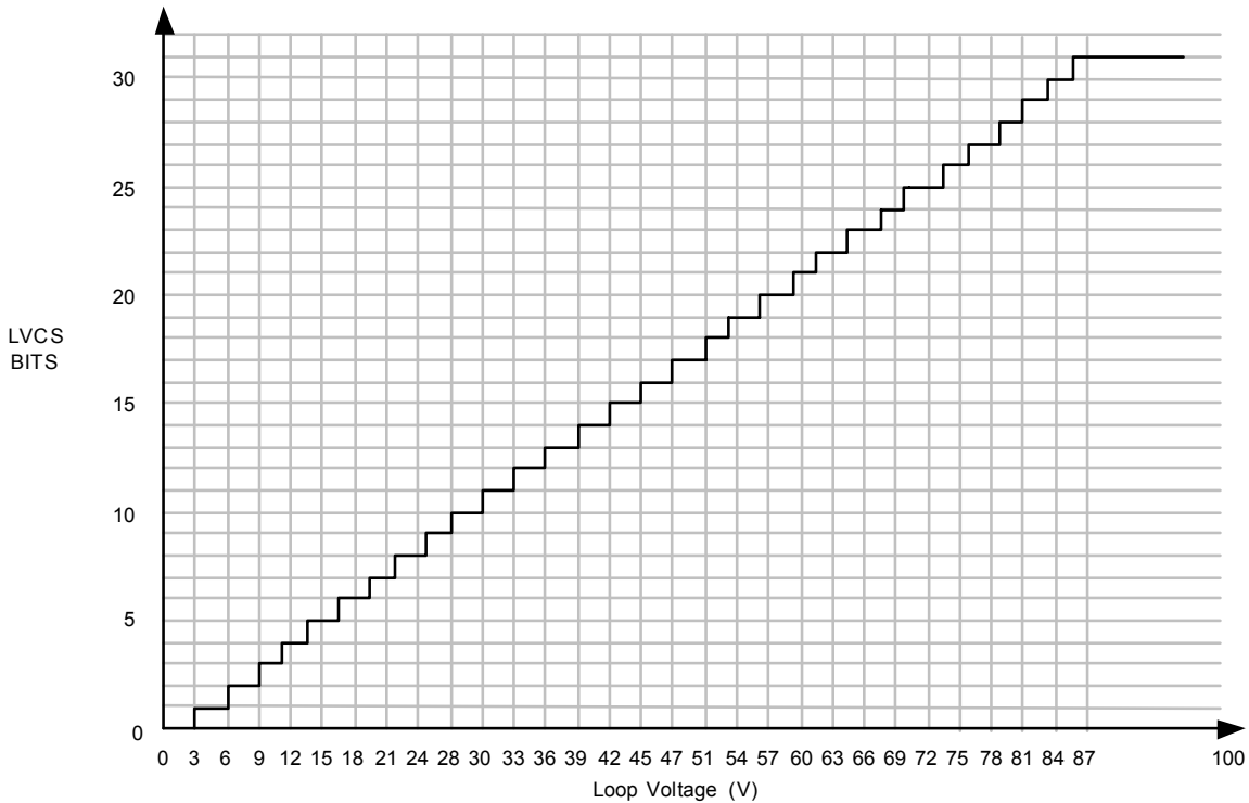
Figure 5. Loop Voltage
