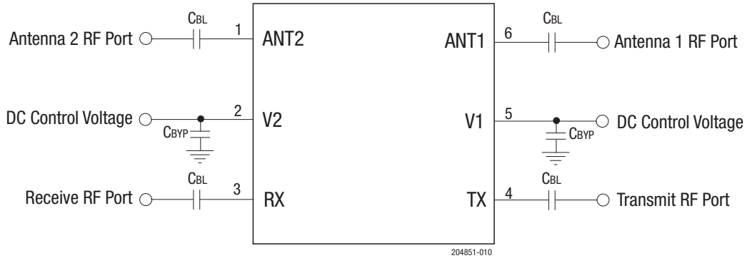
Figure 10. SKYA21070 Evaluation Board Schematic
