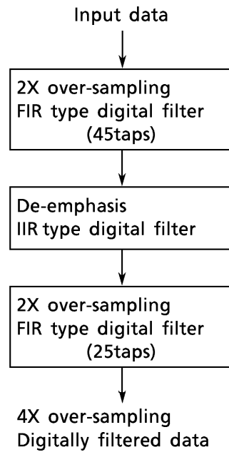
FIG.3 Construction of digital filter
