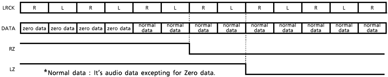
FIG.14 Zero detect cancel timing
