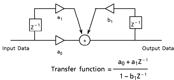
FIG.8 Digital De-emphasis filter construction
