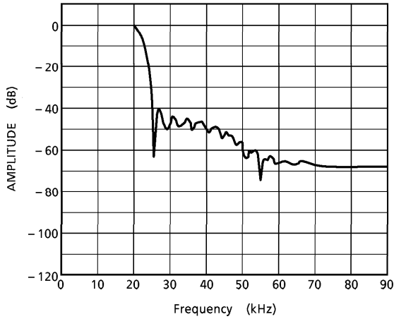
FIG6. Frequency characteristics (stop band)
