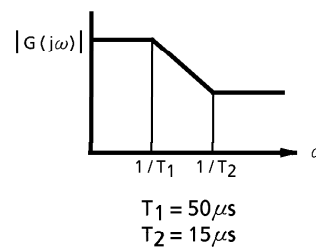
FIG.9 Filter Characteristics
