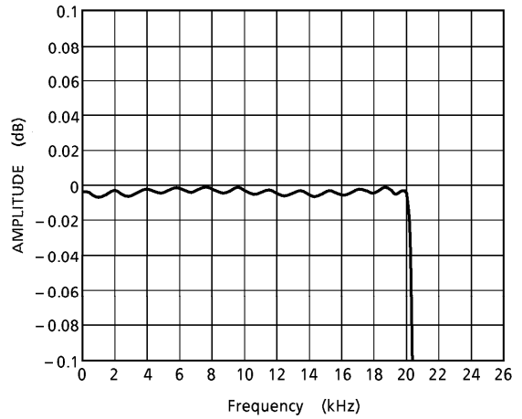
FIG5. Frequency characteristics (pass band)
