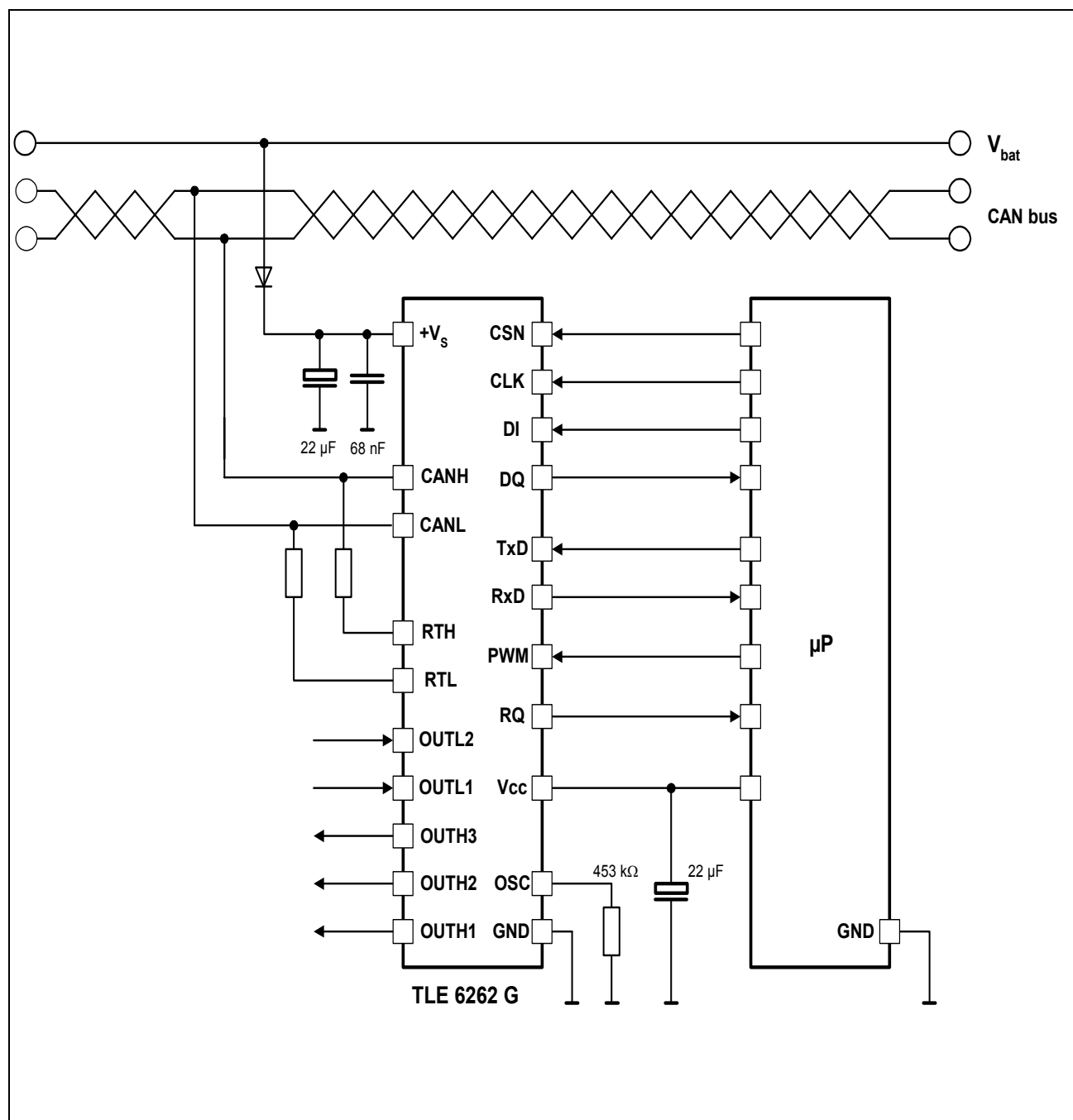
Figure 13 Application Circuit
