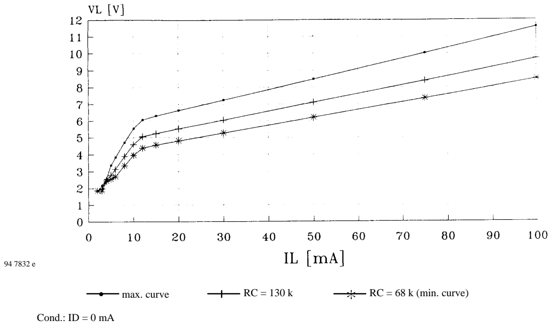
Figure 10. DC characteristics
