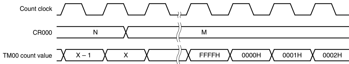
Figure 6-14. Timing After Change of Compare Register During Timer Count Operation (N → M: N &gt; M)
