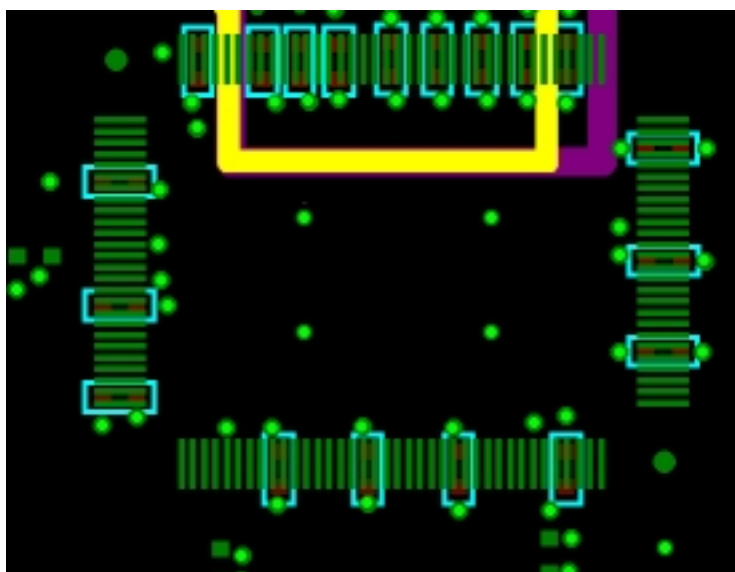
Figure 7. Decoupling Capacitor Placement
