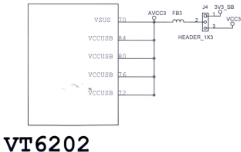
Figure 16. AVCC3 Jumper
