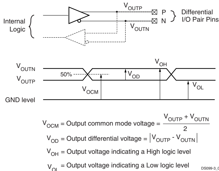
Figure 31: Differential Output Voltages
