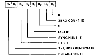
Figure 11. Write Register Bit Functions (Continued)
