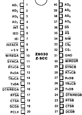
Figure 2. 40-pin Dual-In-Line Package (DIP), Pin Assignments
