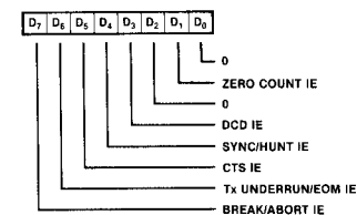
Figure 10. Read Register Bit Functions
