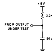
Figure 16. Open-Drain Test Load
