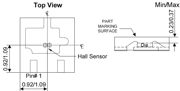
Sensor Location
