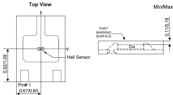
Sensor Location
