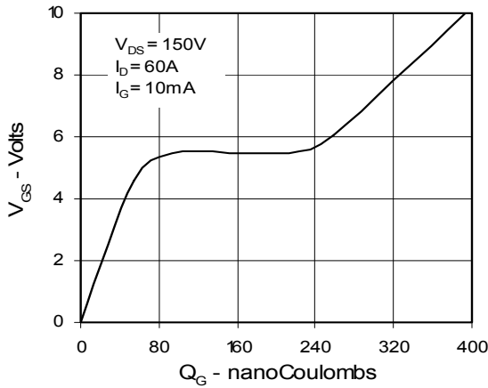
Fig. 9. Gate Charge
